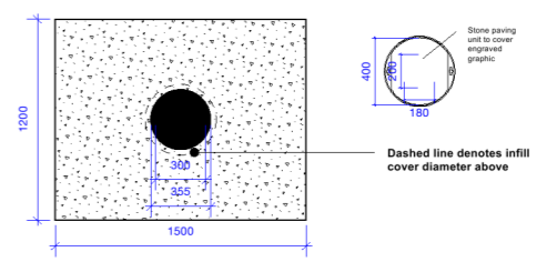
5 Parasol Anchoring Socket - Plan Scale: 1:25
