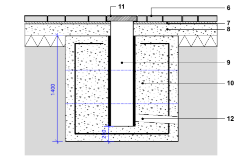
6 Parasol Anchoring Detail Section Scale: 1:25
