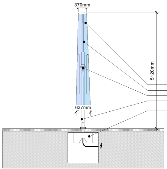
3 Parasol - closed Section Scale: 1:50
